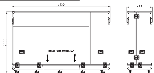
Dimensions of packed Leyard TVF1.5 LED Video Wall with ScreenLifter (in mm):
