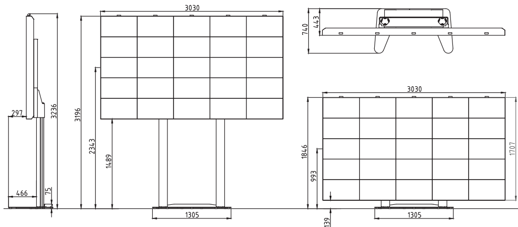
Dimensions of unpacked Leyard TVF1.5 LED Video Wall with ScreenLifter (in mm):
